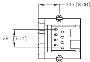
6P4C 6P6C
