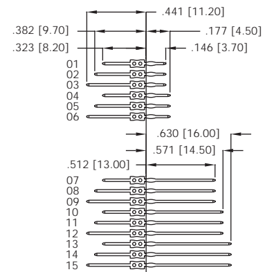
Charts for Customer Use to Designate Pin Lengths
