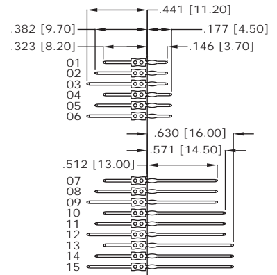
CONTACT DIMENSIONS
