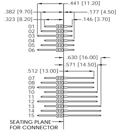
CONTACT DIMENSIONS
