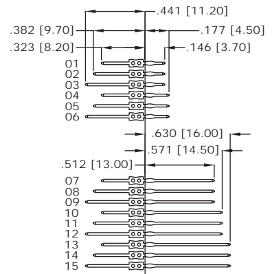
CONTACT DIMENSIONS
